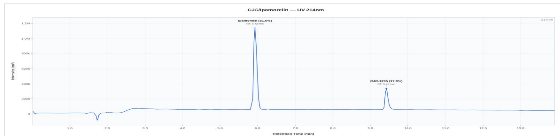
CJC/Ipamorelin 10mg - PC-CI10-001: UV Chromatogram
